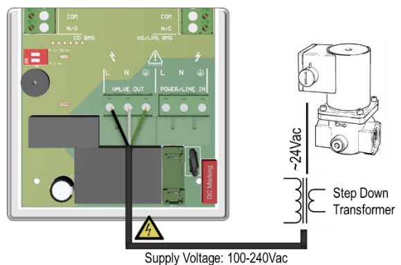
Gas Supply Controlled by 24VAC Solenoid Valve
